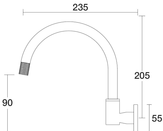
IDK Spa Wall Swivel Outlet D38.044.1.67 - Vintage Brass
