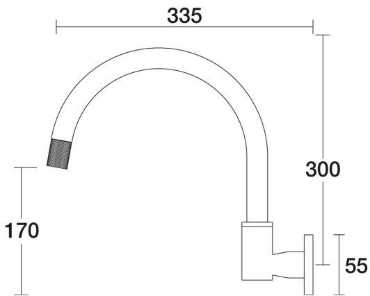
IDK Spa Wall Swivel Outlet X/Large D38.044.2.01 - Chrome
