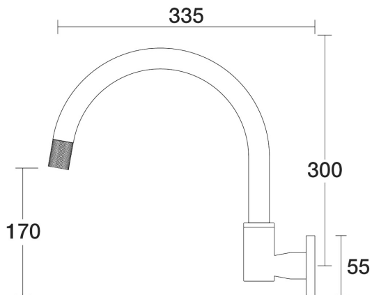
IDK Spa Wall Swivel Outlet X/Large D38.044.2.40 - Rumbled Brass
