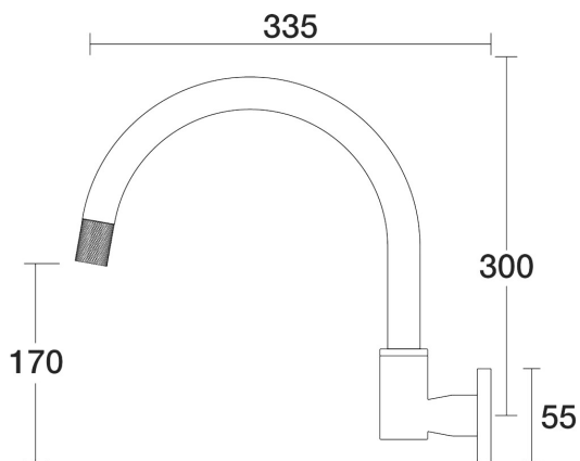
IDK Spa Wall Swivel Outlet X/Large D38.044.2.57 - Matt Nickel
