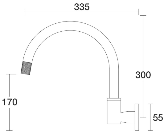
IDK Spa Wall Swivel Outlet X/Large D38.044.2.67 - Vintage Brass
