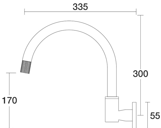
IDK Spa Wall Swivel Outlet X/Large D38.044.2.68 - Autumn Bronze
