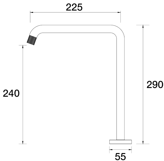
Elm Sink Hob Swivel Outlet D40.032.1.01 - Chrome
