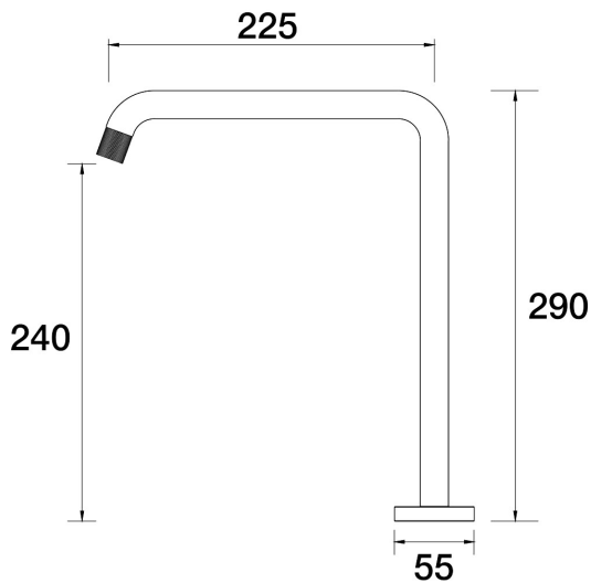
Elm Sink Hob Swivel Outlet D40.032.1.23 - Gunmetal
