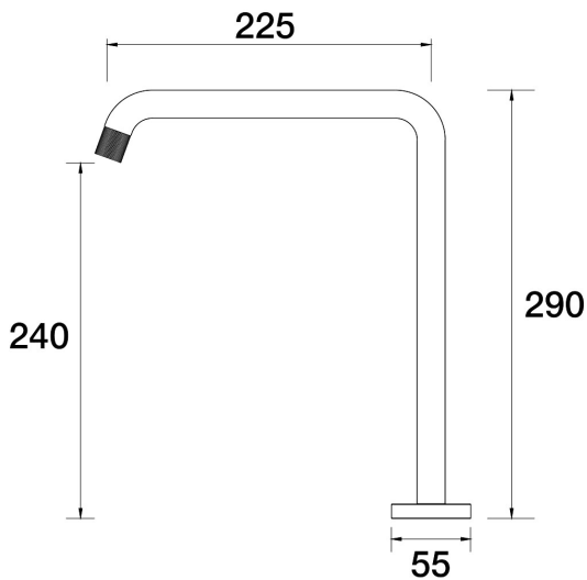
Elm Sink Hob Swivel Outlet D40.032.1.34 - Matt Black
