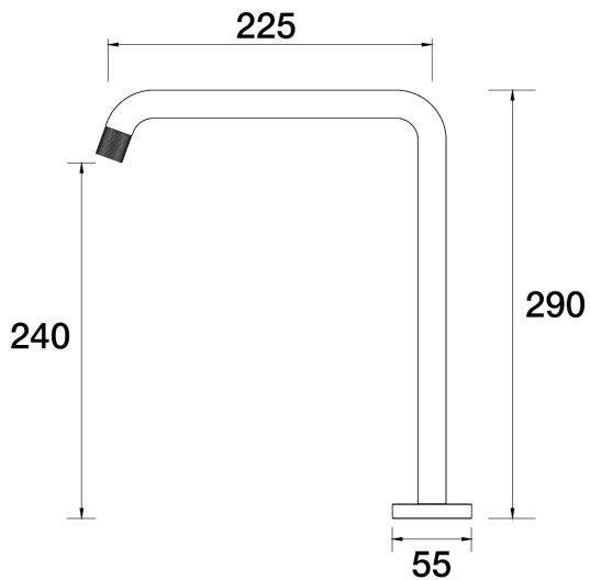
Elm Sink Hob Swivel Outlet D40.032.1.47 - Luminick
