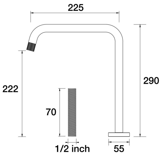
Elm Sink Hob Swivel Outlet For Basin Application ( With Male Nipple) D40.032.2.01 - Chrome
