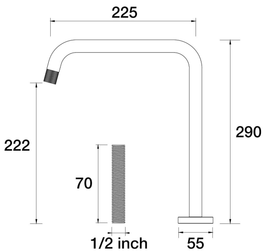
Elm Sink Hob Swivel Outlet For Basin Application ( With Male Nipple) D40.032.2.43 - Brass
