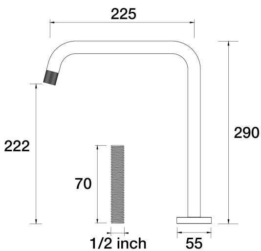
Elm Sink Hob Swivel Outlet For Basin Application ( With Male Nipple) D40.032.2.47 - Luminick
