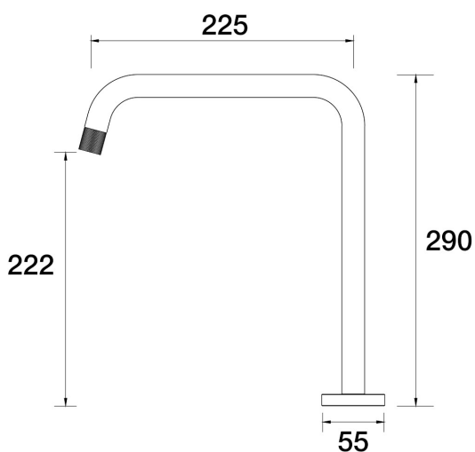
Elm Spa Hob Swivel Outlet D40.042.1.32 - Midnight Black
