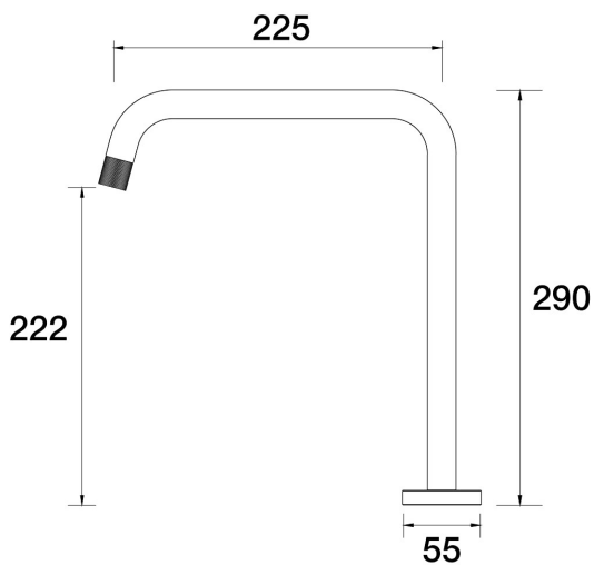
Elm Spa Hob Swivel Outlet D40.042.1.34 - Matt Black
