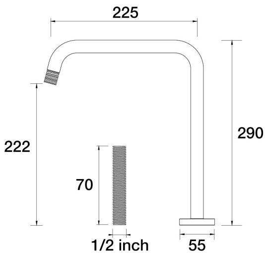
Elm Lane Sink Hob Swivel Outlet For Basin D42.032.2.44 - Antique Copper
