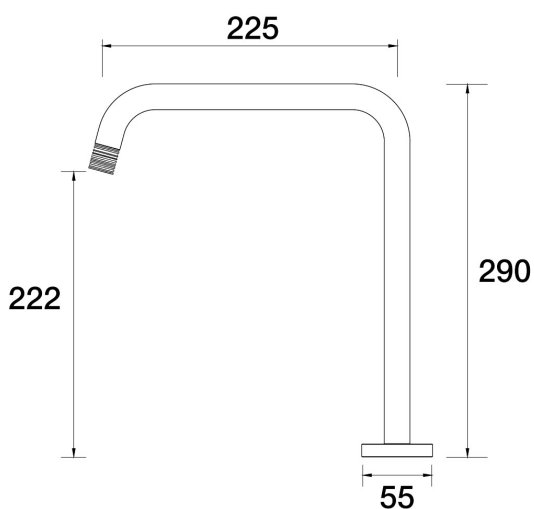
Elm Lane Spa Hob Swivel Outlet D42.042.1.41 - Brushed Brass
