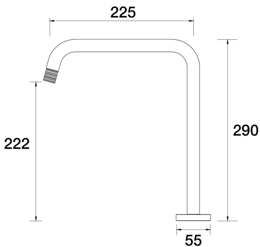
Elm Lane Spa Hob Swivel Outlet D42.042.1.57 - Matt Nickel
