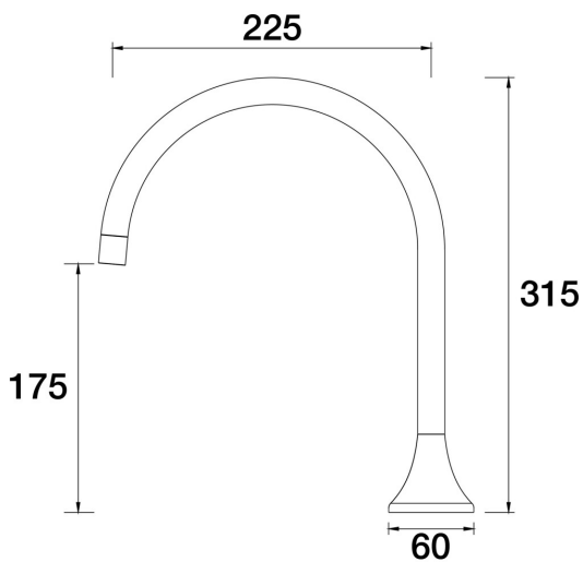
ARI Sink Hob Swivel Outlet D43.032.1.57 - Matt Nickel
