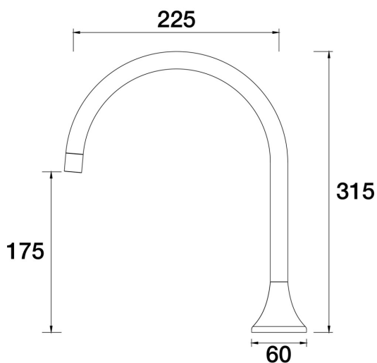
ARI Spa Hob Swivel Outlet D43.042.1.21 - Brushed Rose Gold
