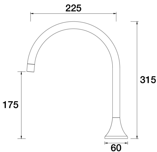
ARI Spa Hob Swivel Outlet D43.042.1.25 - Brushed Nickel
