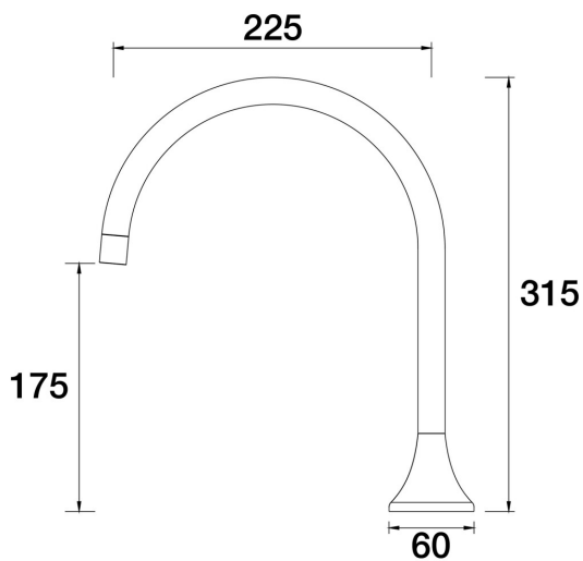
ARI Spa Hob Swivel Outlet D43.042.1.26 - Black Sapphire
