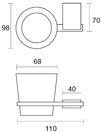
Burj Toothbrush Holder E20.011.1.34 - Matt Black
