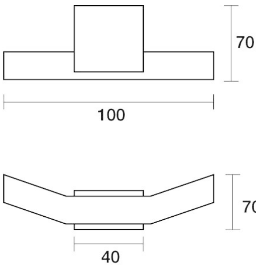
Burj Robe Hook Holder E20.061.1.34 - Matt Black
