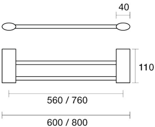
Oracle Towel Rail Double 800mm E21.072.2.34 - Matt Black
