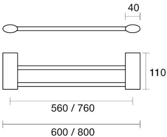
Oracle Towel Rail Double 800mm E21.072.2.41 - Brushed Brass
