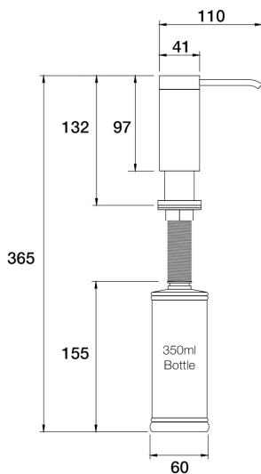
Lugano Soap Pump E22.021.4.41 - Brushed Brass
