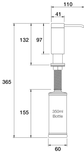
Lugano Soap Pump E22.021.4.67 - Vintage Brass
