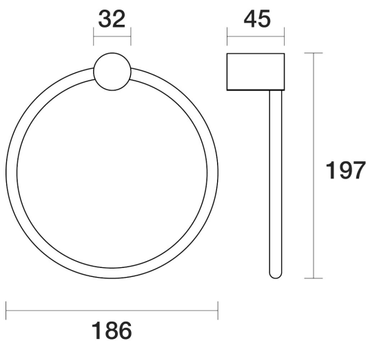
Lugano Towel Ring Holder E22.031.1.57 - Matt Nickel
