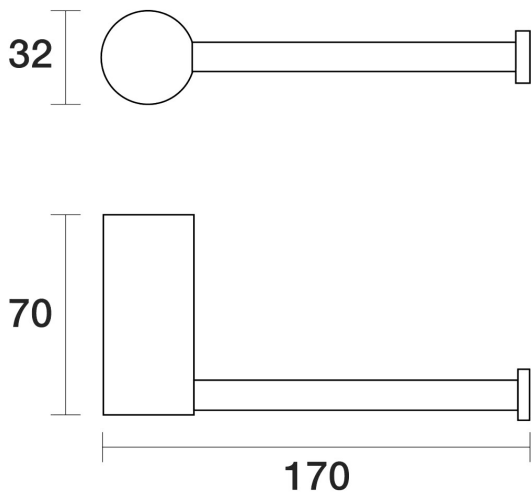
Lugano Toilet Roll Holder E22.051.1.75 - Forest Mist
