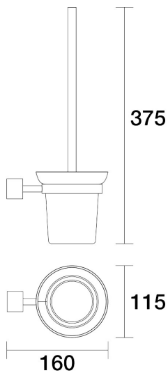
Lugano Toilet Brush Holder E22.052.1.11 - 23k Gold
