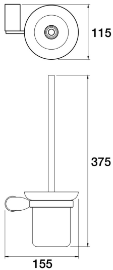
Lava Toilet Brush Holder E23.052.1.41 - Brushed Brass
