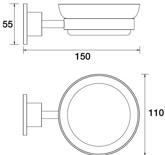
Portsea Soap Dish E29.121.1.01 - Chrome
