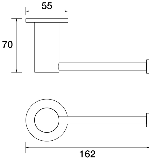
Portsea Toilet Roll Holder Single E29.151.1.11 - 23k Gold
