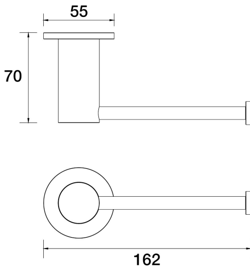
Portsea Toilet Roll Holder Single E29.151.1.47 - Luminick
