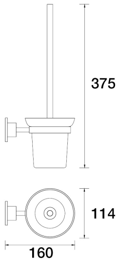
Portsea Toilet Brush Holder E29.152.1.40 - Rumbled Brass
