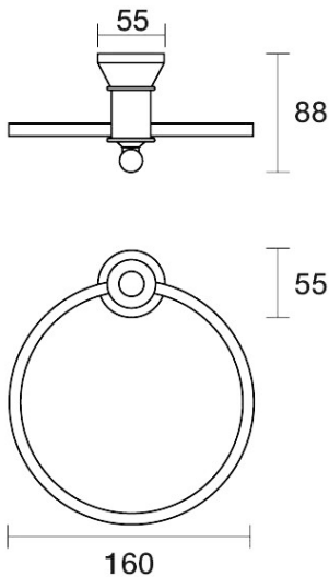
Tudor Towel Ring Holder E31.031.1.02 - Brushed Chrome
