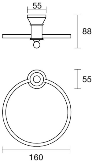
Tudor Towel Ring Holder E31.031.1.26 - Black Sapphire
