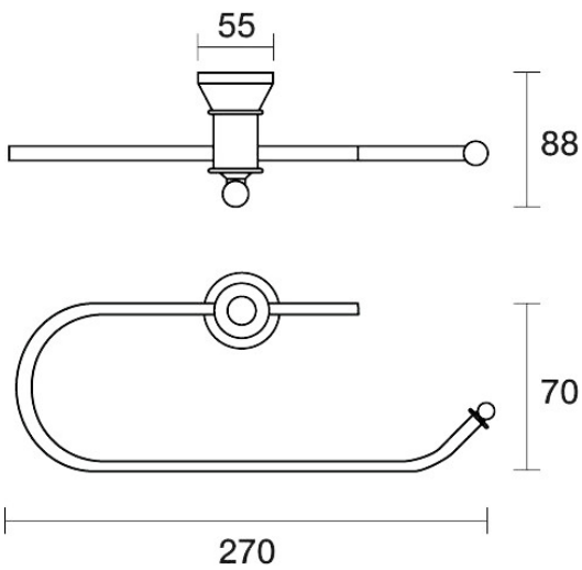
Tudor Guest Towel Holder E31.041.1.19 - 23k Brushed Brass Gold
