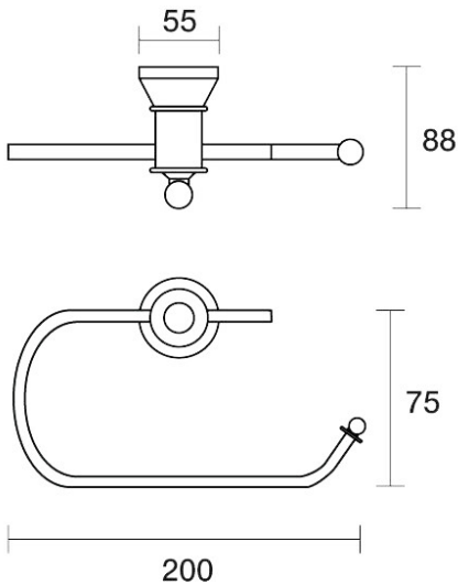
Tudor Toilet Roll Holder E31.051.1.34 - Matt Black
