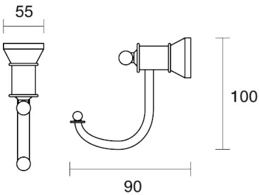
Tudor Robe Hook Holder E31.061.1.57 - Matt Nickel
