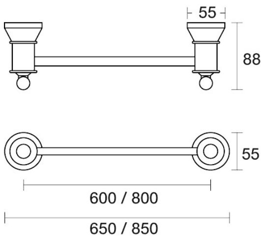
Tudor Towel Rail Single 650mm E31.071.1.03 - Chrome / White
