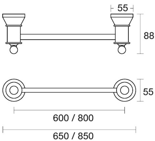
Tudor Towel Rail Single 650mm E31.071.1.13 - Gold / White
