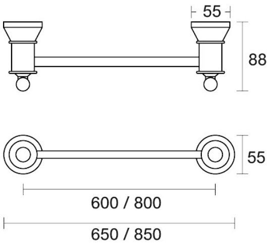
Tudor Towel Rail Single 650mm E31.071.1.39 - Antique Bronze
