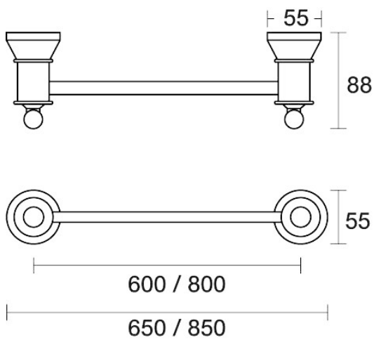
Tudor Towel Rail Single 650mm E31.071.1.41 - Brushed Brass
