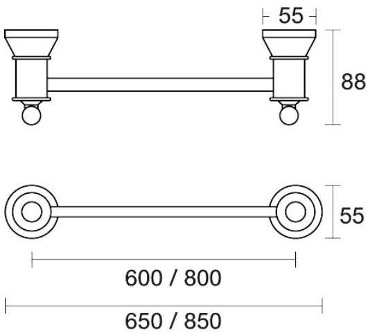
Tudor Towel Rail Single 650mm E31.071.1.52 - Burnished
