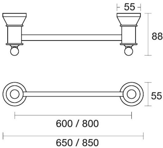
Tudor Towel Rail Single 650mm E31.071.1.57 - Matt Nickel
