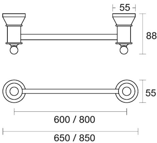
Tudor Towel Rail Single 850mm E31.071.2.27 - Satin Pearl
