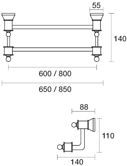
Tudor Towel Rail Double 850mm E31.072.2.06 - Chrome / Sienna Red
