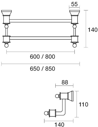
Tudor Towel Rail Double 850mm E31.072.2.24 - Brushed Gunmetal
